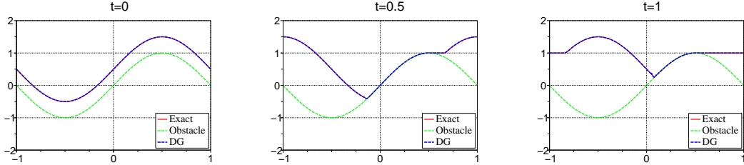
FIGURE 1. Example 1, RKDG scheme, times t = 0 , t = 0.5 and t = 1 , using P^2 elements with N_x = 20 mesh cells (obstacle : green dotted line).
