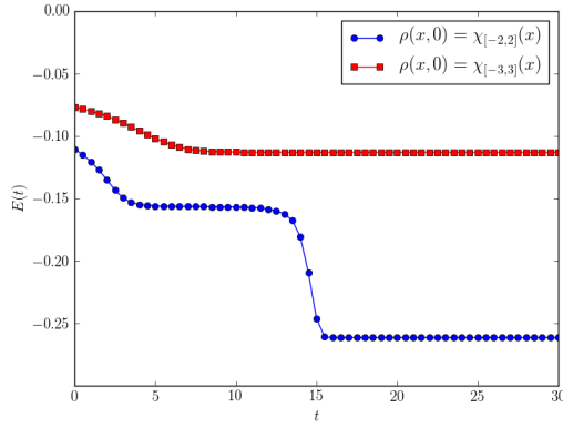
(a) Entropy
