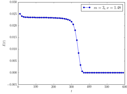
(a) Entropy.
