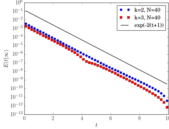
Figure 4.3: The relative entropy for porous equation, with \rho(x, 0) = \max\{1 - |x - \frac{1}{2}|, 0\} .
