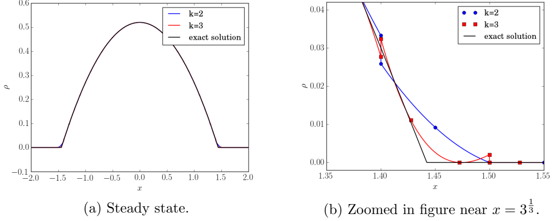
Figure 4.1: Profiles of the numerical steady states for (4.2.1), with \rho(x, 0) = \max\{1 - |x|, 0\} .
