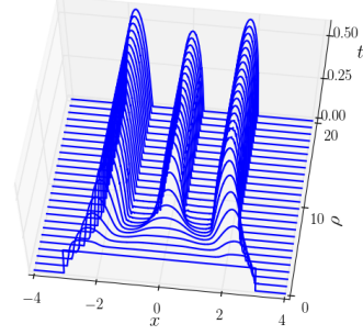
(b) \rho(x, 0) = \chi_{[-3,3]}(x)
