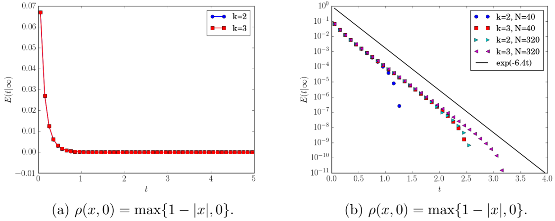
Figure 4.2: The entropy and the relative entropy for (4.2.1), with \rho(x, 0) = \max\{1 - |x|, 0\} .
