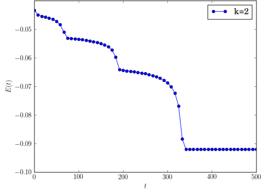
(a) Entropy.
