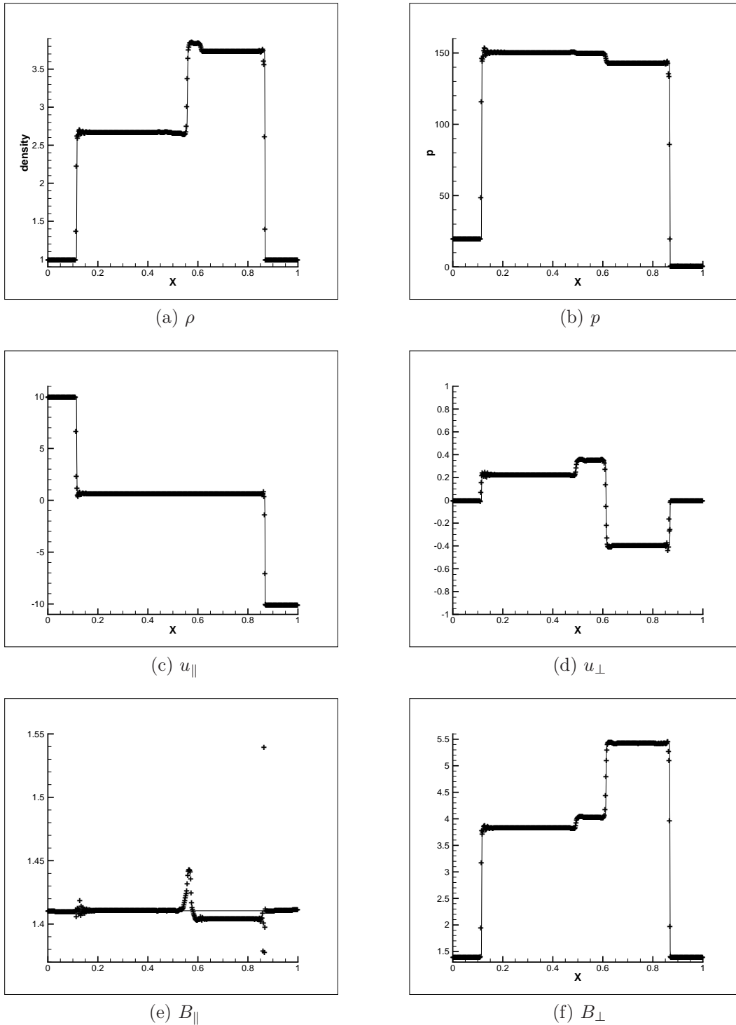
Fig. 4.7: The solution of the 2D rotated shock tube problem by the entropy stable DG scheme (symbols) on a mesh with 512 \times 2 cells. For comparison, the non-rotated 1D solution with 800 cells is also plotted (solid line).
