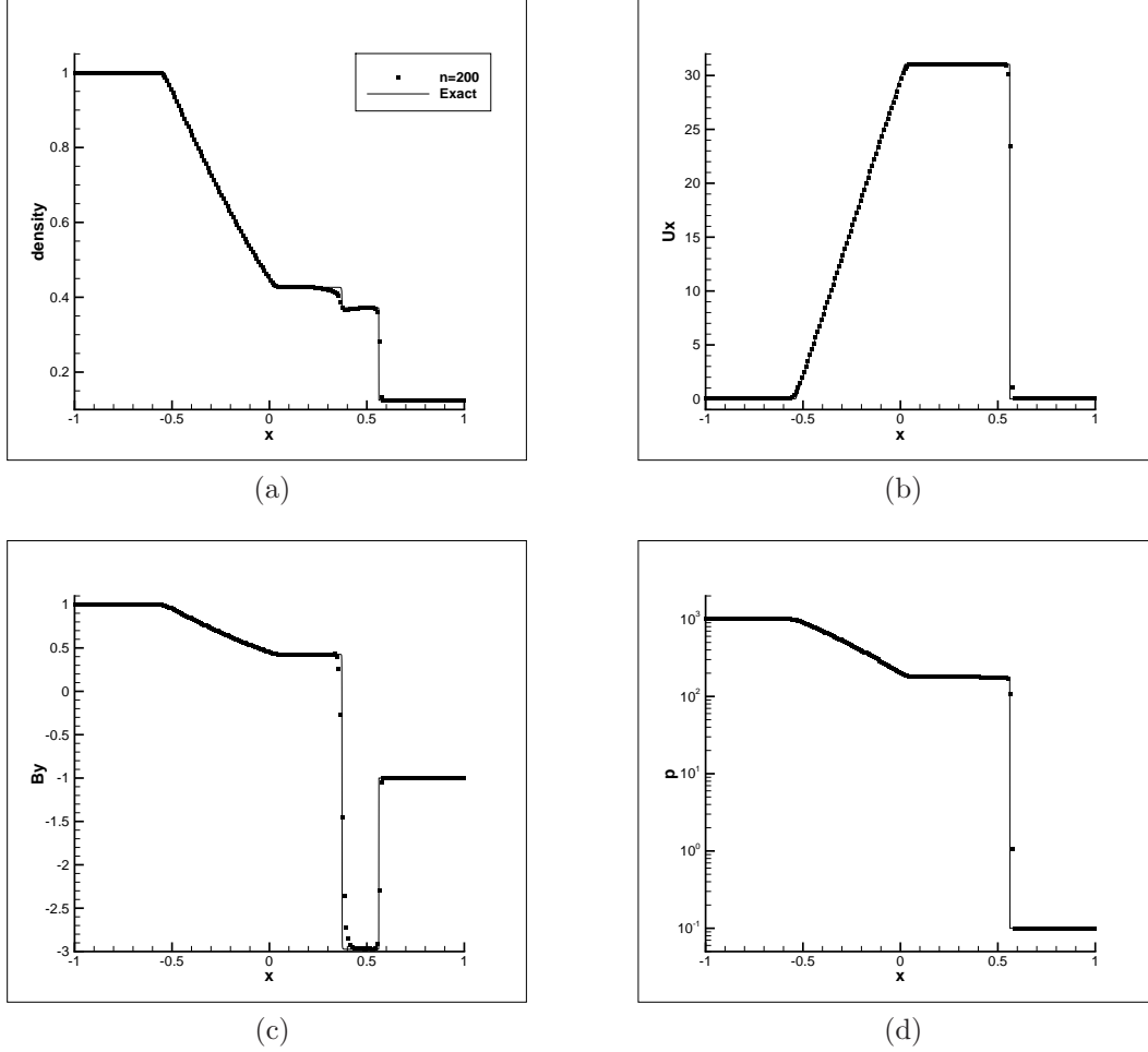
Fig. 4.2: The second one-dimensional Riemann example with 200 cells (squares) on a background solid line of the exact solution. t = 0.012 and M = 10 . Top left : \rho ; top right: u_x ; bottom left: B_y ; bottom right: p .
