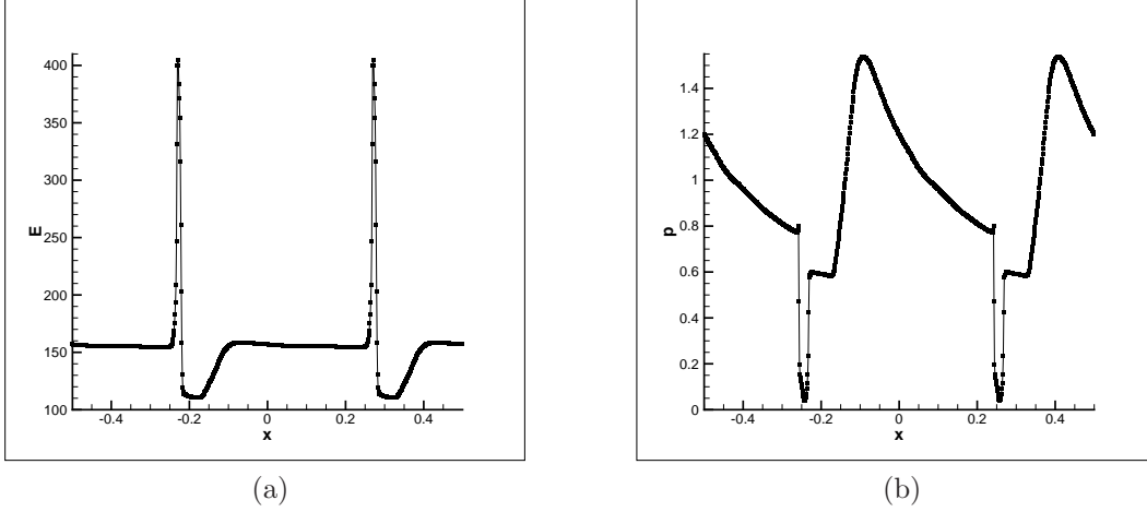
Fig. 4.3: The total energy E (left) and pressure p (right) of the torsional Alfvén wave pulse on an 800 cell mesh at t = 0.156
