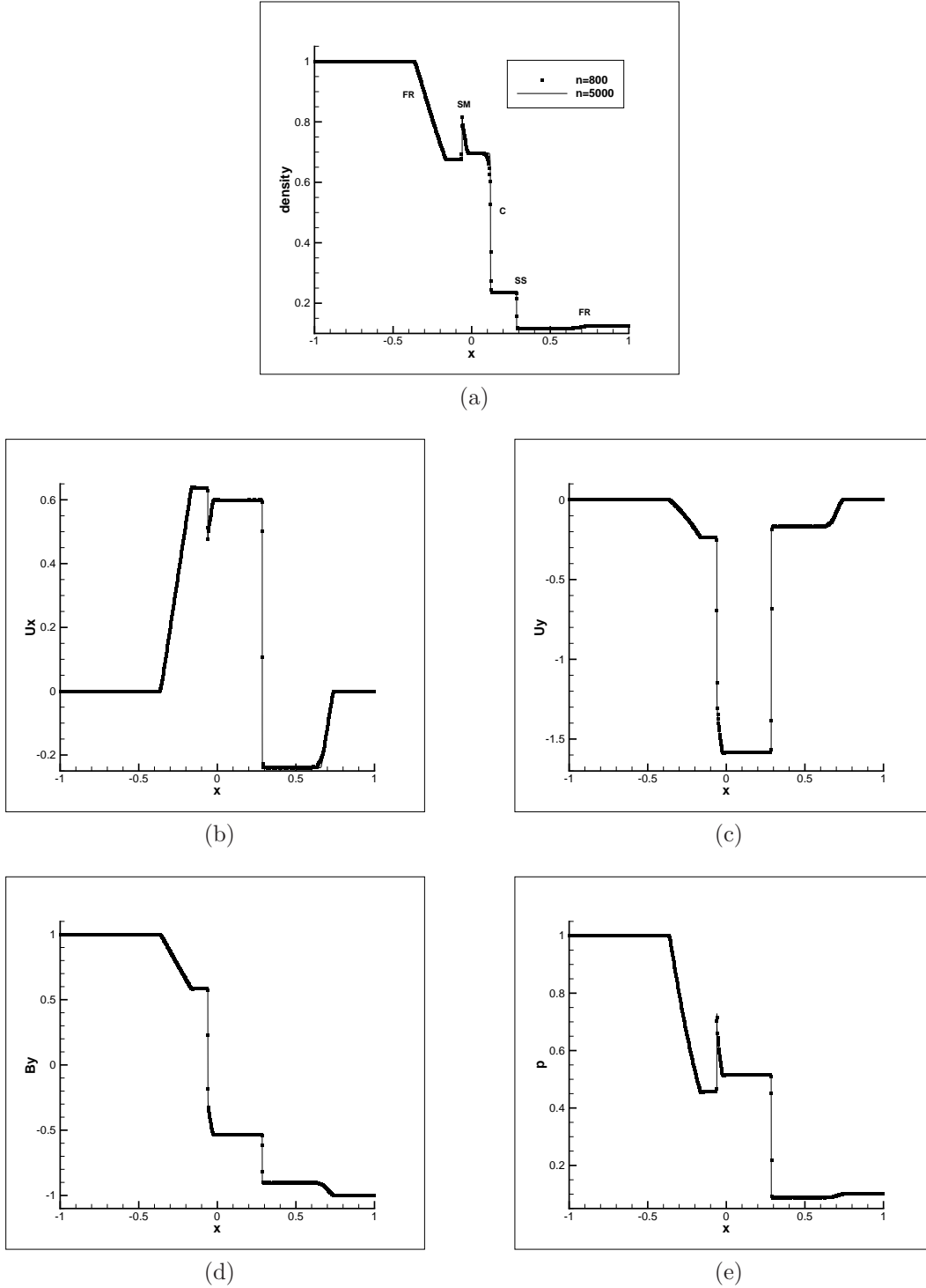
Fig. 4.1: The first one-dimensional Riemann example with 800 cells (squares) on a background solid line computed with 5000 cells. t = 0.2 and M = 10 . The symbol FR denotes a fast rarefaction wave; SM is a compound wave (an intermediate shock followed by a slow rarefaction wave); C is a contact discontinuity; SS is a slow shock. Top: \rho ; middle left: u_x ; middle right: u_y ; bottom left: B_y ; bottom right: p .
