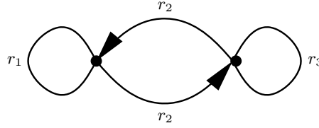
Figure 2. \mathcal{I} -weighted stable curve of type [4] \times^2 [4] .
