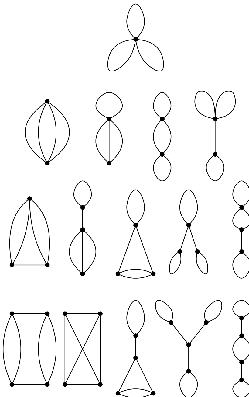
Figure 1. Stable curves with arithmetic genus 3 and geometric genus zero.
