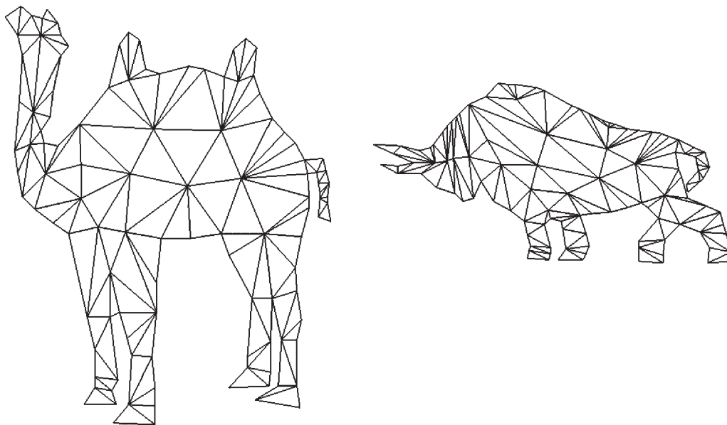
Figure 8. Isomorphic meshes.
