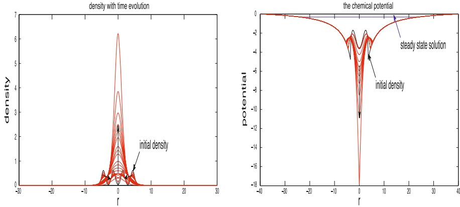
Fig. 3. Time evolution of the density (left) and the chemical potential (right). Blow-up for the supercritical case 2d/(d+2) < m < 2 - 2/d , p = \frac{d(2-m)}{2} , the initial data is non-decreasing with two maximums and satisfies \|U_0\|_p > \|U_s\|_p , the solution will blow up at a finite time T and its chemical potential has a negative minimum at the blow-up position as t \rightarrow T
