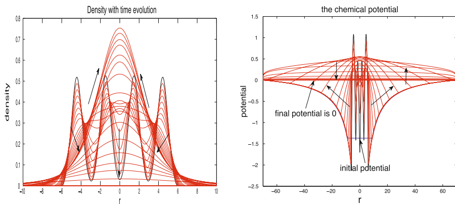
Fig. 2. Time evolution of the density (left) and the chemical potential (right). Spreading for the supercritical case 2d/(d+2) < m < 2 - 2/d , p = \frac{d(2-m)}{2} . Here the initial data has two maximums and satisfies C_{d,m} < \|U_0\|_p < \|U_s\|_p , the solution will spread out to the whole space and decays to zero, and its chemical potential also tend to zero as t \rightarrow \infty
