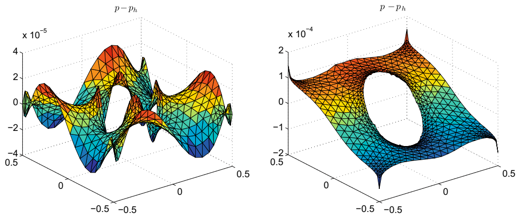
Fig. 6. Pressure error in the square with hole for the (3,2) PA (left) and SC (right) scheme. \Delta t = 0.02 . 1296 P4 elements for each variable. T = 2 . Only values at the vertices of triangles are used in the plots.
