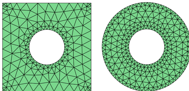
Fig. 5. Finite-element meshes for stability and temporal accuracy checks. Square with hole: \{(x,y) | r^2 \leq x^2 + y^2 \leq R^2, |x|, |y| \leq R\} . Annulus: \{(x,y) | r^2 \leq x^2 + y^2 \leq R^2\} . (r,R) = (0.2,0.5) .
