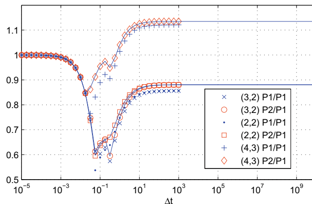
Fig. 1. Largest magnitude of eigenvalue vs. \Delta t . PA scheme. Thirty elements for each variable. Solid lines are theoretical results from Appendix A.
