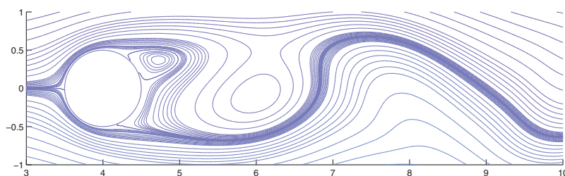
FIG. 5.16. \text{Re} = 100 , T = 45 .
