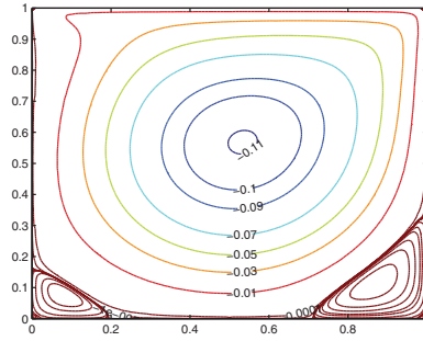
FIG. 5.2. Streamline, Re = 1000.
