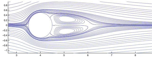
FIG. 5.14. \text{Re} = 40 , T = 10 .
