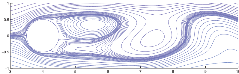
FIG. 5.15. \text{Re} = 100 , T = 35 .
