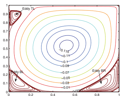
FIG. 5.7. Streamline , Re = 5000 .
