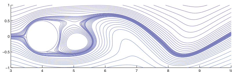
FIG. 5.17. \text{Re} = 100 , T = 60 .
