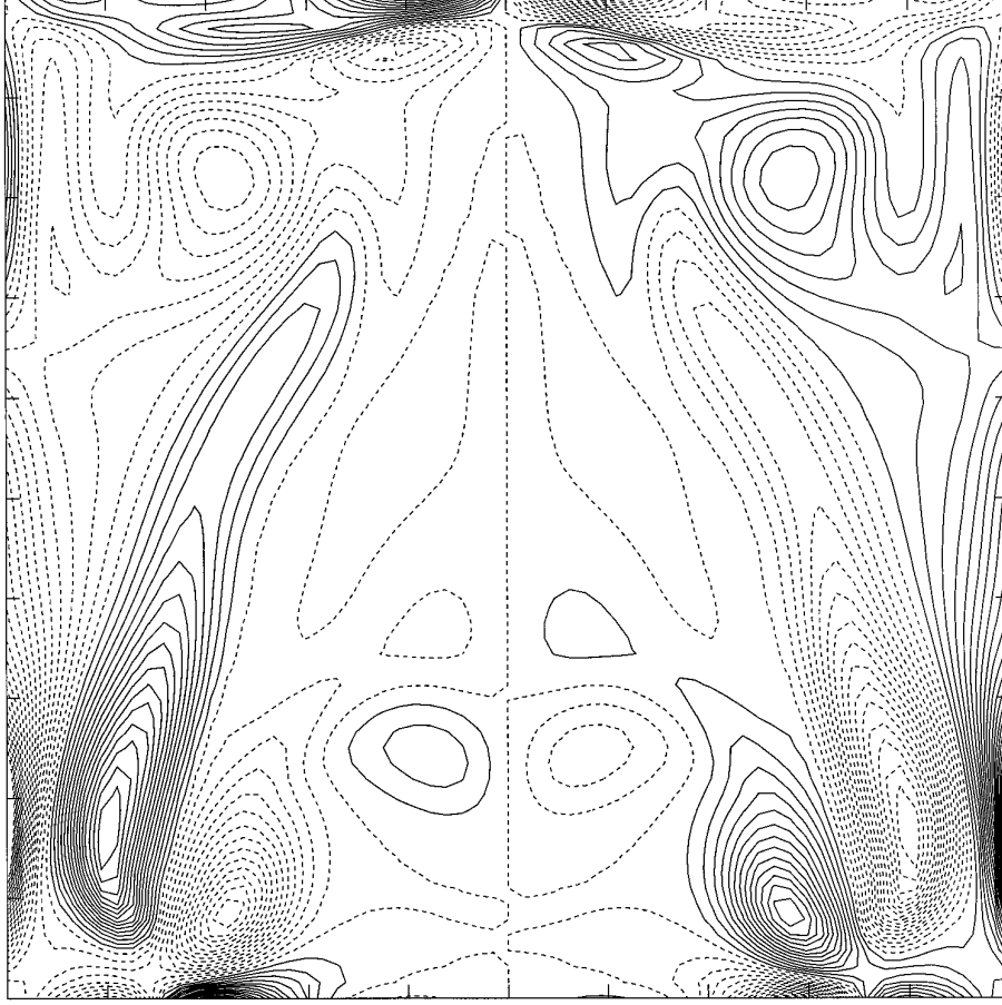
FIG. 10. Contour plot of \omega_1 at the center plane \{x = \frac{1}{2}\} computed using Method B and (4.1). Parameters: Re = 3200 , t = 15 , CFL = \Delta t/\Delta x = 2.5 , \Delta x = \frac{1}{64} .
