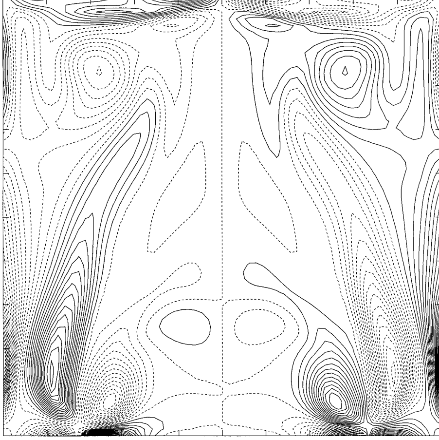
FIG. 13. Contour plot of \omega_i at the center plane \{x = \frac{1}{2}\} computed using Method A and (4.1). Parameters: \text{Re} = 3200 , t = 15 , CFL = \Delta t/\Delta x = 2.5 , \Delta x = \frac{1}{64} .
