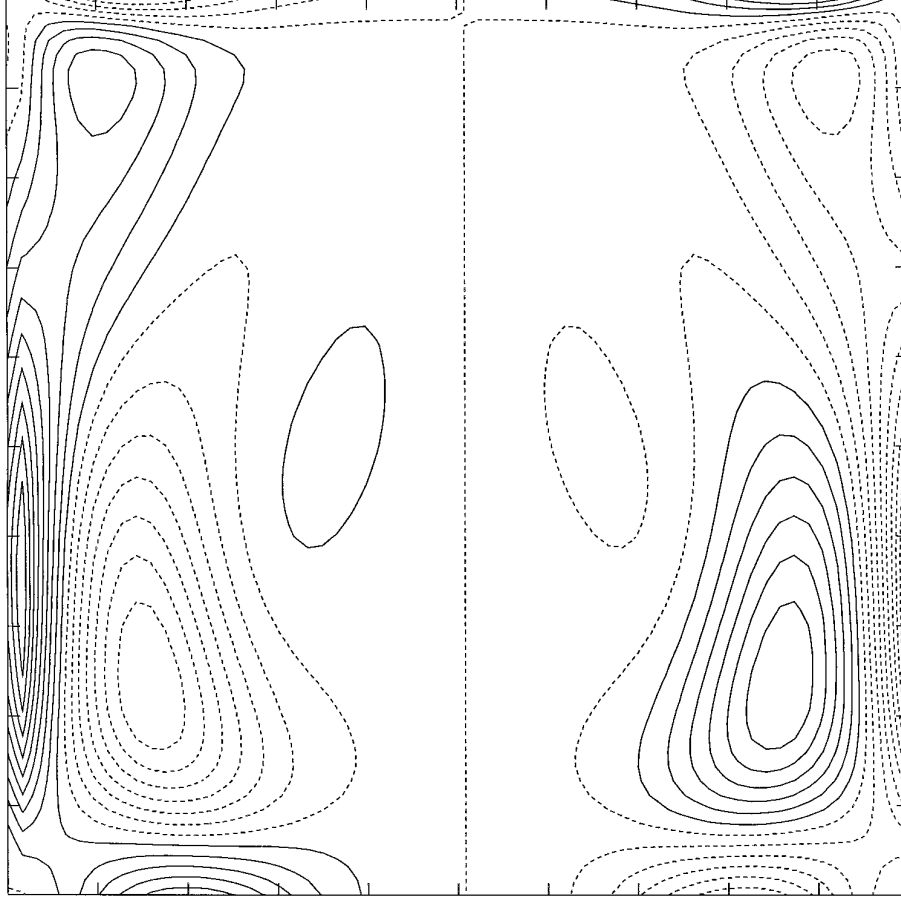
FIG. 6. Contour plot of \omega_1 at the center plane \{x = \frac{1}{2}\} computed using MAC scheme. Parameters: \text{Re} = 500 , t = 20 , CFL = \Delta t/\Delta x = 2.5 , \Delta x = \frac{1}{32} .
