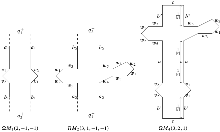
Figure 13. Smoothing two pairs of simple poles.
