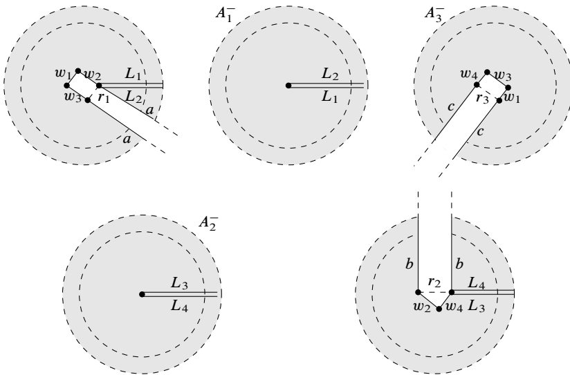
Figure 15. Bottom level flat surface Z inside \Omega\mathcal{M}_1(8, -2, -3, -3) .
