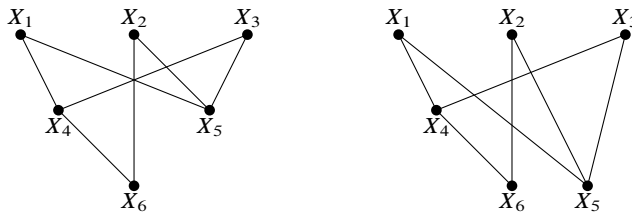
Figure 5. Two level graphs \bar{\Gamma}_1 and \bar{\Gamma}_2 used in Example 3.4.
