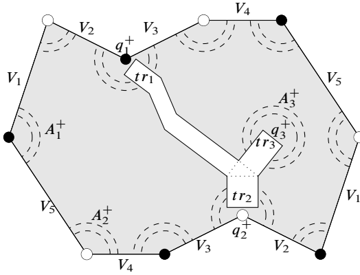
Figure 14. Top level flat surface Y inside \Omega\mathcal{M}_2(1, 1, 0) .
