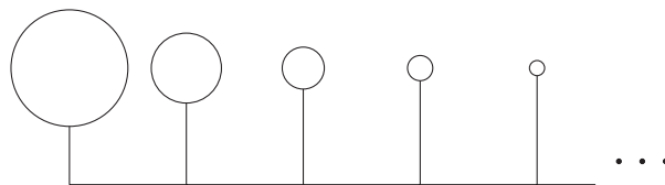
Figure 2. A metric space with zero covering radius
