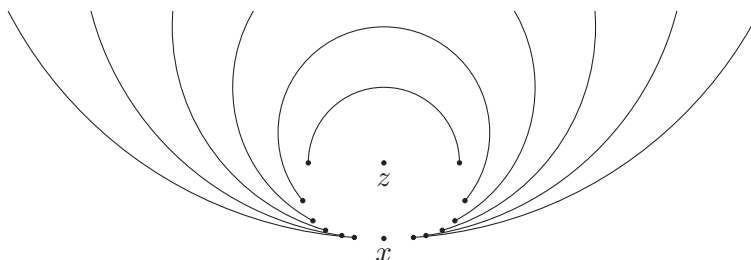
Figure 3. A metric space with infinite covering radius
