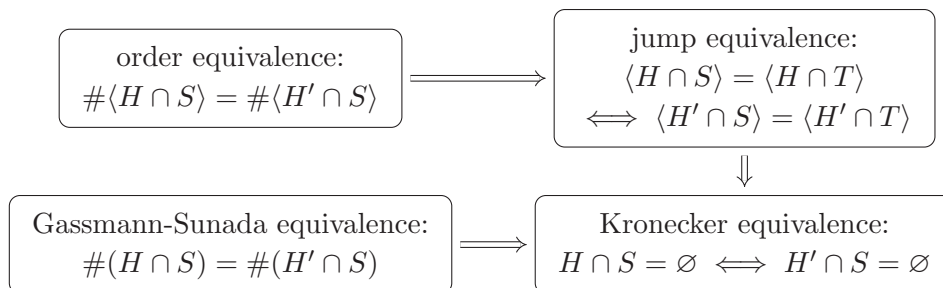
Figure 4. Notions of equivalence
