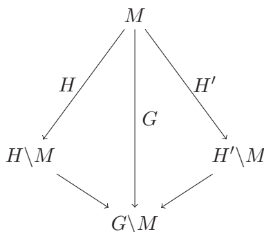
Figure 1. Diagram of Covering Spaces
