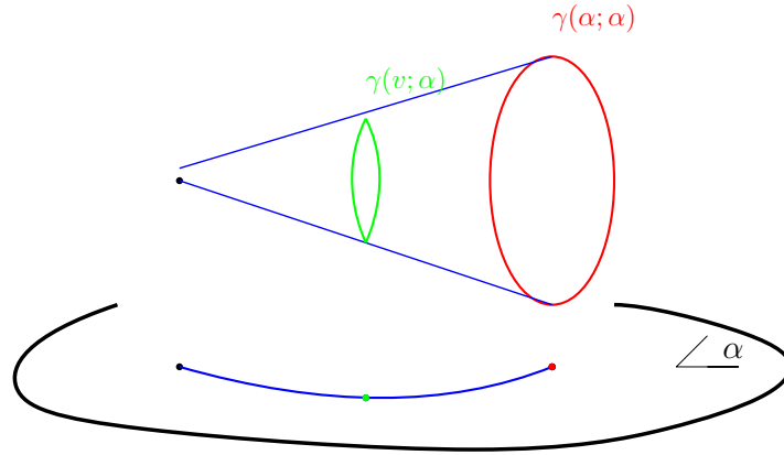
Figure 2: Thimble swept out by singular cycles.
