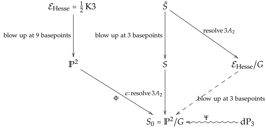
Figure 6: Blow-up geometries enjoying nice arithmetic properties.
