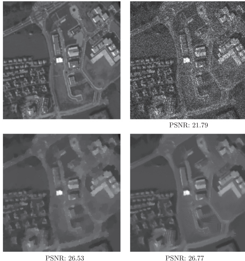
Figure 5. Top: parts of the images depicted in figure 4 (left and middle). Bottom: restored images by the I -divergence constrained model (16) with total variation seminorm (left) and the nonlocal term ( p = 17, \omega = 17, a = 4 ) (right), respectively.
