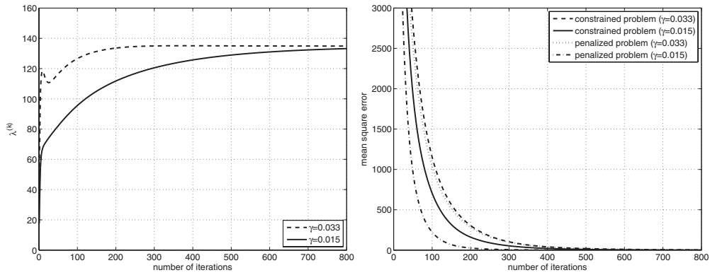
Figure 2. Convergence speed of x^{(k)} and \lambda^{(k)} in algorithm I when computing the restored image in figure 1 (right). Left: iterates \lambda^{(k)} for different parameters \gamma . Right: evolution of the mean-square errors \frac{1}{\lambda} \|x^{(k)} - x^*\|_2^2 between the intermediate results x^{(k)} and a sufficiently converged reference result x^* .
