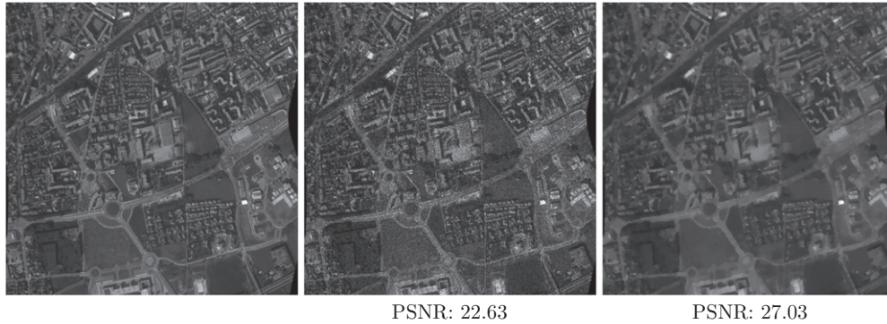
Figure 4. Left: Original image of the French city of Nîmes ( 512 \times 512 ) with values in the range [1, 256] , see also [35]. Middle: image corrupted by multiplicative Gamma noise ( K = 10 ). Right: restoration result by the I -divergence constrained model (16) with total variation seminorm ( \gamma = 0.015 ).
