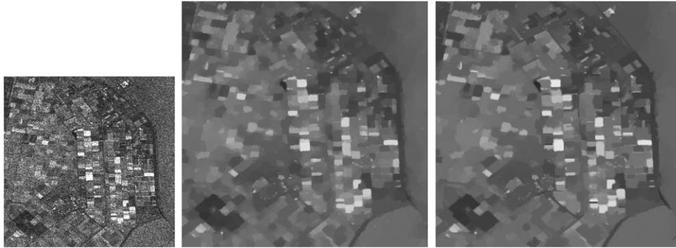
Figure 6. Left: real multi-look SAR image (copyright by [37]) of size 512 \times 512 with values in [0, 255] . Middle: restoration result by the I -divergence constrained model (16) with the total variation seminorm applied to the squared image. Right: result by the I -divergence constrained model (16) with the nonlocal term ( l = 9, \omega = 13, a = 3 ) applied to the squared image.
