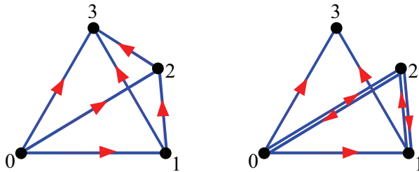
Figure 3: Star-like digraphs
