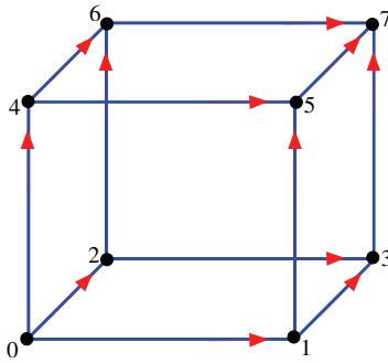
Figure 2: 3-cube
