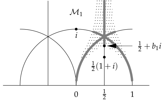
Figure 4. The dotted region is the lifted domain \tilde{\Omega}_5 \subset F_0 . The lower boundary curve C_1 \ni \frac{1}{2} + b_1 i consists of \tau with \frac{1}{2}\omega_1 being a degenerate critical point of G . The upper left (resp. right) boundary is C_3 (resp. C_2 ) respectively.
