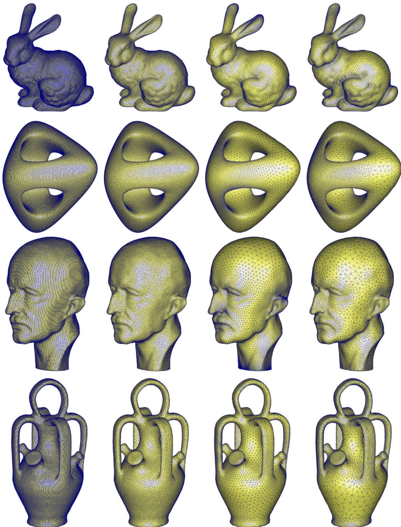
Fig. 11. Results of isosurface sampling/meshing on synthetic data. Left: MC; middle left: uniform MPS; middle right: AF; right: adaptive MPS. Here, MC refers to the marching cubes algorithm [1], MPS refers to our algorithm with uniform sampling, AF refers to the advancing front approach [5], and AMPS refers to our algorithm with adaptive sampling.
