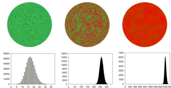
Fig. 5. Uniform sampling on a sphere. From left to right: The neighborhood sizes of the analysis are 0.005, 0.02, and 0.05. See the caption of Fig. 4 for an explanation.
