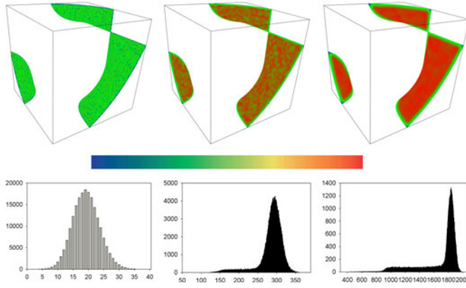
Fig. 4. Uniform sampling inside a unit cube. The isovalues at the vertices are \{-3, 3, 1, -1, 2, -1, 12, 1\} . Left: d = 0.005 ; middle: d = 0.02 ; right: d = 0.05 . The color-coding indicates the number of neighboring samples inside a sphere centered at each sample point, where green indicates a smaller value and red indicates a larger value. The histograms show the distribution of neighborhood sizes where neighborhood size is defined by the number of points inside it. The flat regions in the histogram stem from the points on the boundaries.
