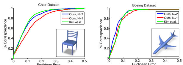
Fig. 14. Comparison of Euclidean error distribution with [31].
