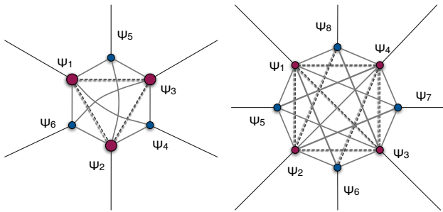
FIG. 1. Finite approximation to the reflectionless scale invariant vertices corresponding to (16) (left) and (18) (right) constructed according to (10)–(11). Dotted line indicates the presence of a non-zero phase shift \chi_{ij} .
