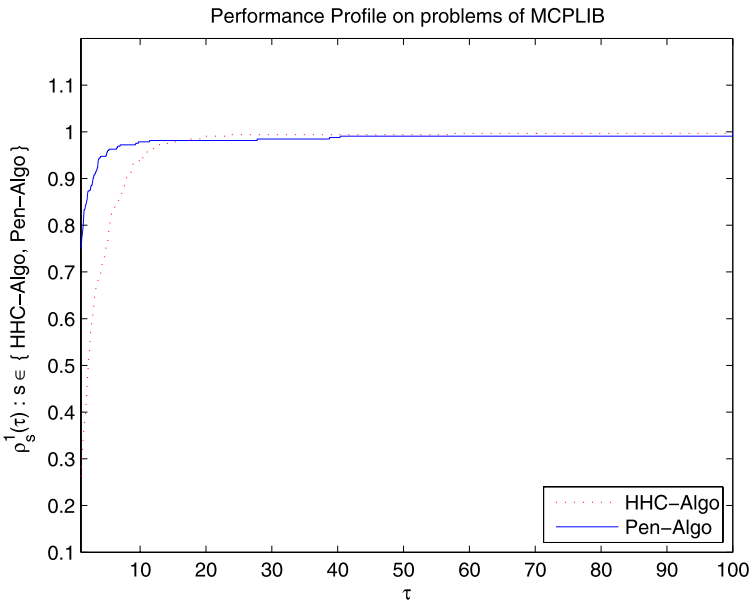
Fig. 2 Performance profile with respect to iterative number: global
