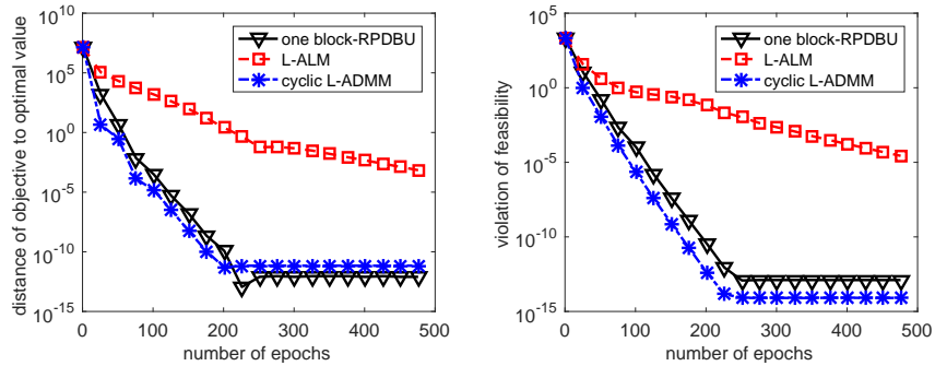
Figure 2: Comparison of the proposed method (RPDBU) to the linearized augmented Lagrangian method (L-ALM) and the cyclic linearized alternating direction method of multipliers (L-ADMM) on solving the nonnegativity constrained quadratic programming (56). Left: distance of objective to optimal value |F(x^k) - F(x^*)| ; Right: violation of feasibility \|Ax^k - b\| .
