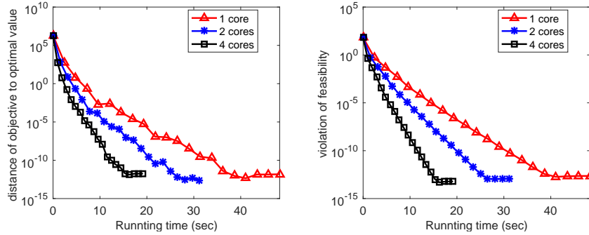
Figure 1: Nearly linear speed-up performance of the proposed primal-dual method for solving (56) on a 4-core machine. Left: distance of objective to optimal value |F(x^k) - F(x^*)| ; Right: violation of feasibility \|Ax^k - b\| .
