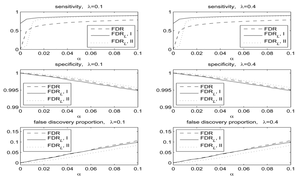
Fig 5. Comparison of the average sensitivity (top panels), average specificity (middle panels) and average false discovery proportion (bottom panels). Left panels: \lambda = 0.1 . Right panels: \lambda = 0.4 .
