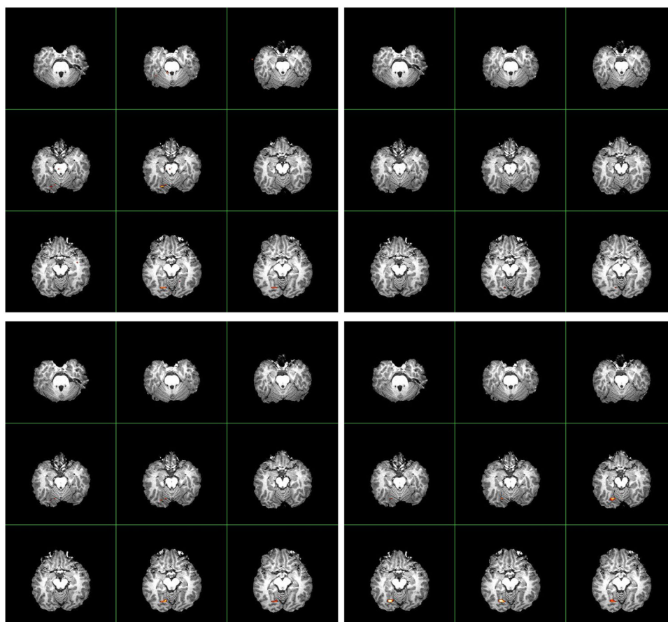
Fig 8. Comparison of activated brain regions detected for the simulated fMRI dataset using the conventional FDR approach (on the left) and the proposed FDR_L procedure (on the right) using Method I. Top panels: AFNI. Bottom panels: FSL. Here \alpha = .05 .
