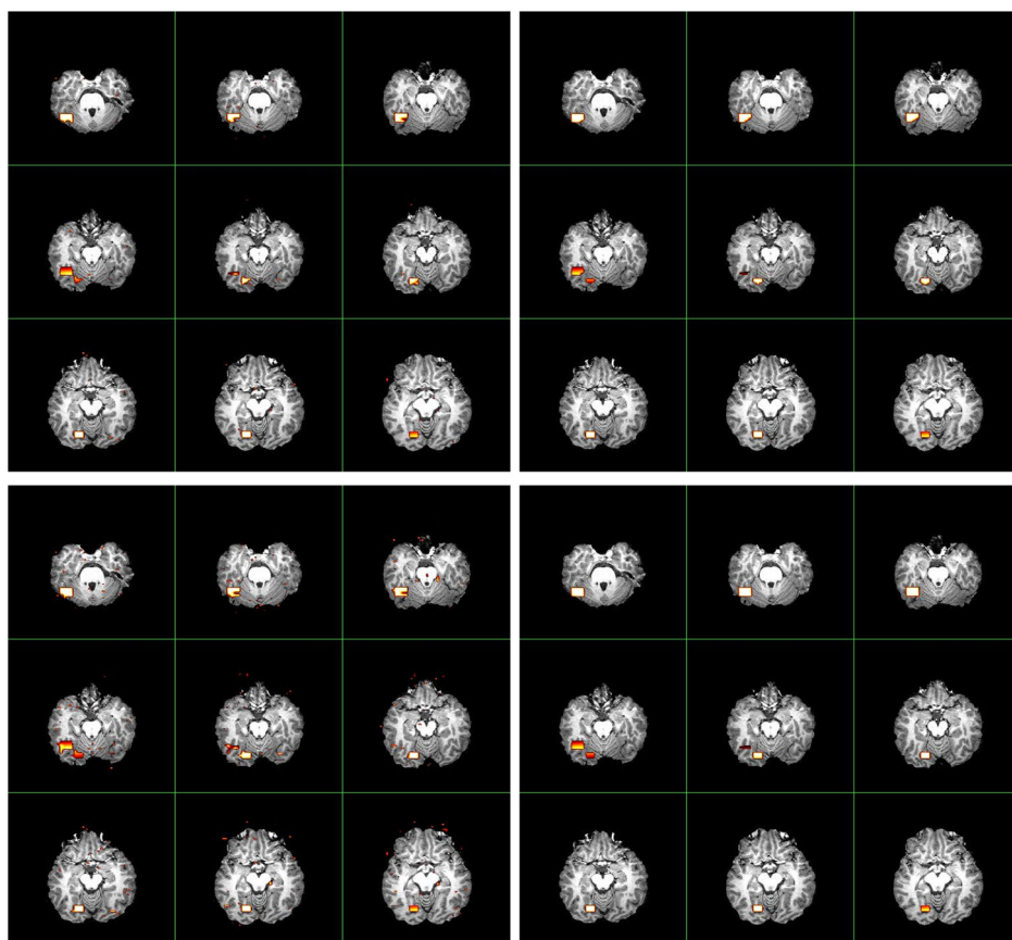
Fig 7. Comparison of activated brain regions detected for the simulated fMRI dataset using the conventional FDR approach (on the left) and the proposed FDR_L procedure (on the right) using Method I. Top panels: K . Bottom panels: K_{be} . Here \alpha = .05 .
