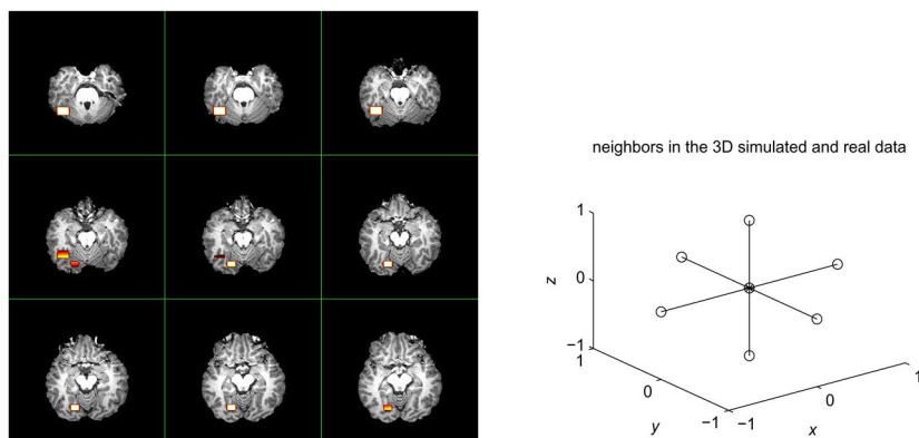
Fig 6. Left panel: true activated brain regions (denoted by hot color) for the simulated fMRI dataset. Right panel: neighbors of a point at (x,y,z) used in the FDR_L procedure for 3D simulated and real data.
