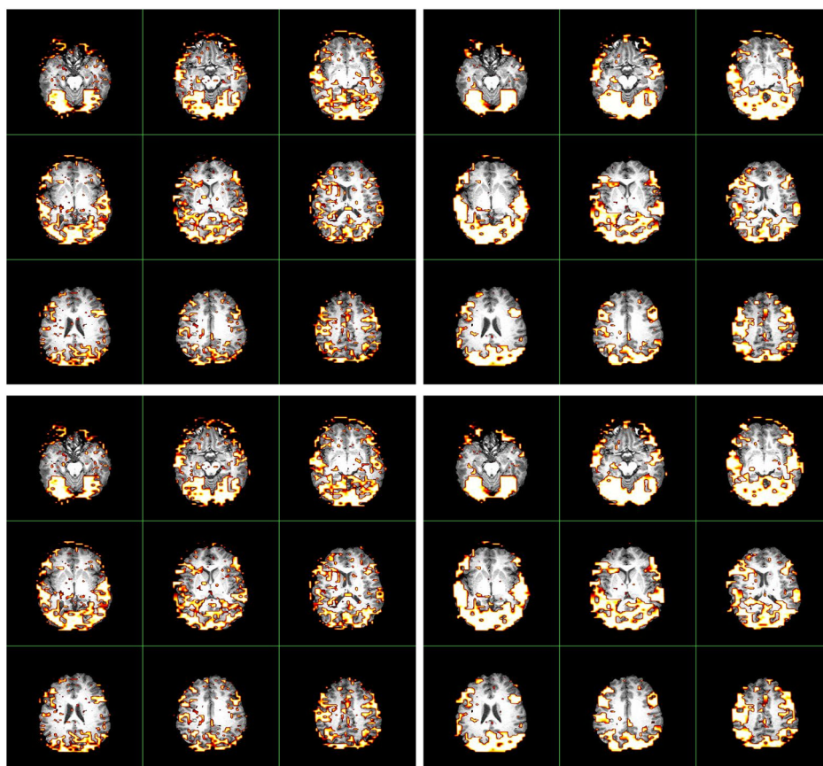
Fig 9. Comparison of activated brain regions detected for the real fMRI dataset using the conventional FDR approach (on the left) and the proposed FDR_L procedure (on the right) using Method I. Top panels: K . Bottom panels: K_{be} . Here \alpha = .001 .
