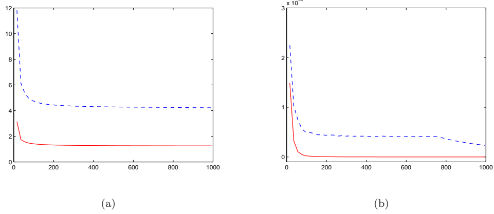
Figure 3: (a) The MSEs of estimated variances of the optimal portfolios with \gamma_n = 10\% over 500 simulations based on \hat{\Sigma} (solid curve) and \hat{\Sigma}_{\text{sam}} (dashed curve) against p . (b) The MSEs of estimated global minimum variances over 500 simulations based on \hat{\Sigma} (solid curve) and \hat{\Sigma}_{\text{sam}} (dashed curve) against p .
