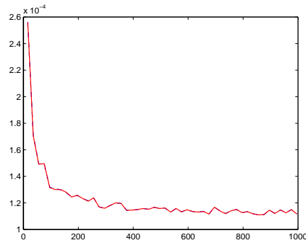
Figure 4: The MSEs of estimated variances of the equally weighted portfolio over 500 simulations based on \hat{\Sigma} (solid curve) and \hat{\Sigma}_{\text{sam}} (dashed curve) against p .
