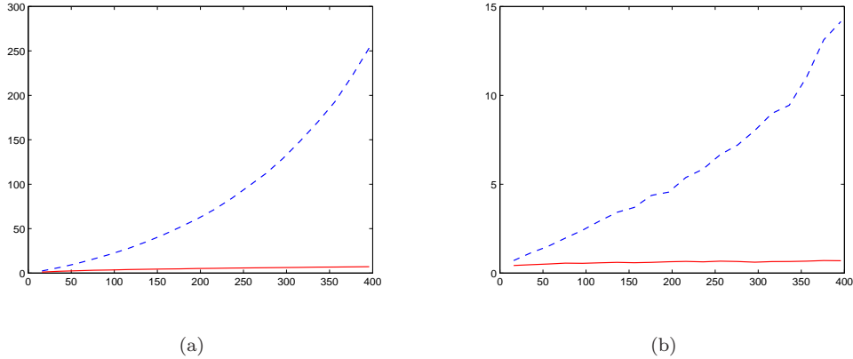
Figure 2: (a) The averages of errors under Frobenius norm over 500 simulations for \hat{\Sigma}^{-1} (solid curve) and \hat{\Sigma}_{\text{sam}}^{-1} (dashed curve) against p . (b) Corresponding standard deviations of errors under Frobenius norm.
