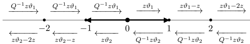
FIGURE 1. \mathcal{M}_{\text{red}}(\Sigma_{\mathbb{P}^1})
