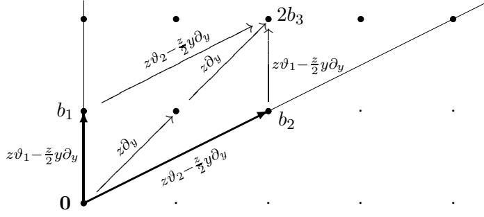
FIGURE 3. \mathcal{M}_{\text{red}}(\Sigma_{[\mathbb{C}^2/\mu_2]}, \{(1, 1)\})
