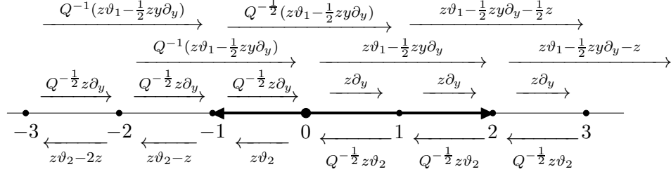
FIGURE 2. \mathcal{M}_{\text{red}}(\Sigma_{\mathbb{P}(1,2)}, \{1\})
