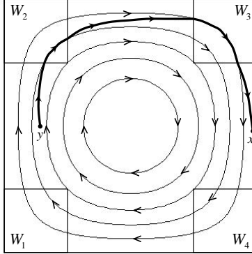
Figure 3: An illustration of a controlled trajectory \eta connecting two points in the quarter cell (enclosing a single vortex) of the cellular flow in the proof of Lemma 3.3. The quarter cell (large square) containing the closed streamlines is [0, \pi]^2 , the smaller squares in the four corners are of size \pi/4 by \pi/4 .
