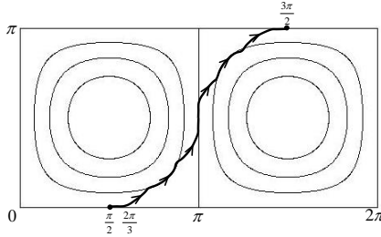
Figure 2: An illustration of a controlled trajectory \xi traveling between two vortices of the cellular flow in the proof of Lemma 3.1.
