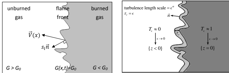
Figure 1: Left: G-equation model Right: Majda-Souganidis model
