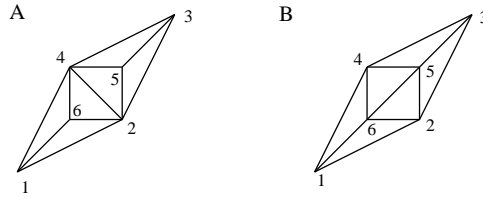
Fig. 3: Two phases of a local Calabi-Yau manifold. Phase B is obtained by a flop transition.
