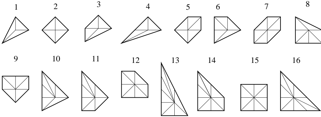
Fig. 1: Reflexive Polyhedra ( \Delta_B ) in two dimensions. \hat{\Delta}_p = \Delta_{17-p} for p = 1, \dots, 6 . \Delta_{7,8,9,10} are self-dual [37][24] 17 . Case one is the polyhedron representing the \mathbf{P}^2 ; two, three and four are the Hirzebruch surfaces F_0 = \mathbf{P}^1 \times \mathbf{P}^1 , F_1 and F_2 and the others are various blow-ups of these cases. Note that c_2 = \#2 simpl. and c_1^2 = 12 - \#2 simpl. The labeling starts with 0 for the inner point. The point to its right is point 1 and the labels of the others increase counterclockwise.
