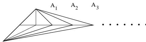
Fig. 2: Toric diagrams ( \Delta_B ) for the A_n singularity fibered over \mathbf{P}^1 . Note that these diagrams have unique triangulations.
