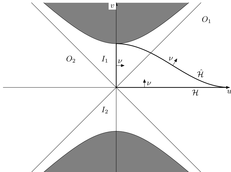
Figure 4: Kruskal Coordinates
