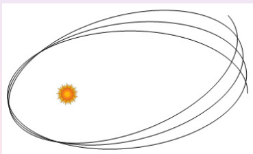
Perihelion of mercury
