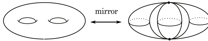
Figure 9: Genus 2 curve and mirror perverse curve
