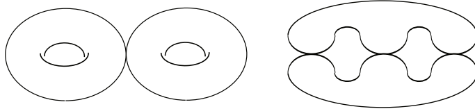
Figure 7: Conifold loci and large complex structure limit
