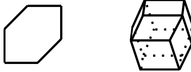
Figure 10: 2 and 3-dimensional zonotopes
