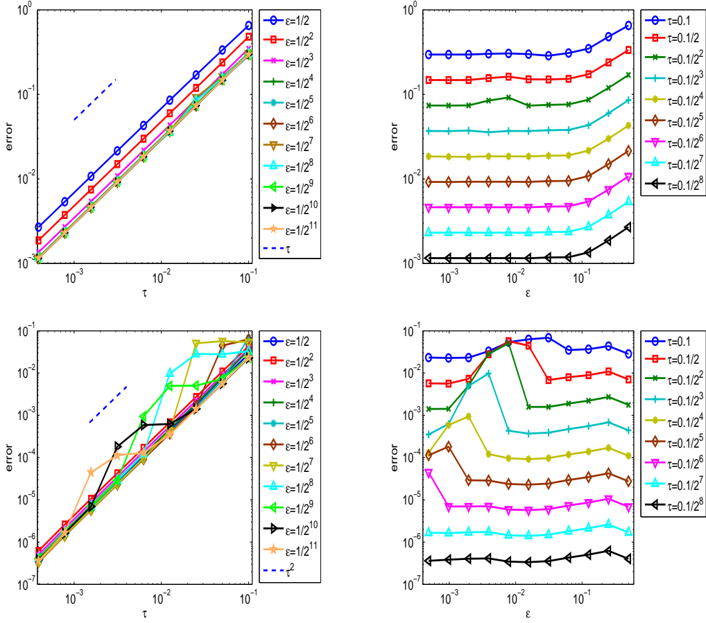
FIGURE 2. Error \|u(\cdot, t_n) - u^n\|_{H^1} + \|\partial_t u(\cdot, t_n) - \dot{u}^n\|_{H^1} at t = 2 of the Lie-Trotter splitting (above) and Strang splitting (below) for the KGE-OP (2.8) under different \epsilon and \tau .
