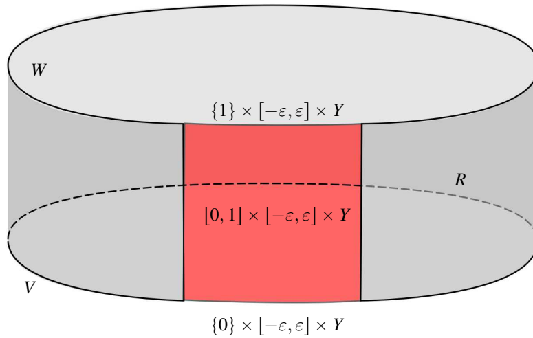
Figure 1: The spin cobordism
