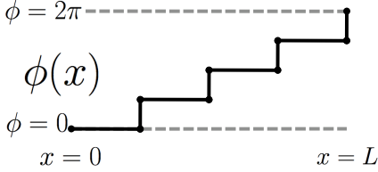
FIG. 5: A nontrivial winding \int_0^L dx \partial_x \phi(x) = 2\pi . This is like a soliton (or particle) insertion. For N_{12} number of Z_{N_1} -symmetry breaking domain walls, we predict that the integer p_{21} units of total induced Z_{N_2} charge on a 1D ring. In average, each kink captures a p_{21}/N_{12} fractional units of Z_{N_2} charge.
