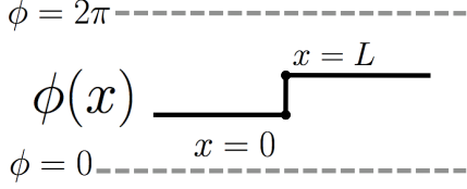
FIG. 4: We expect some fractional charge trapped near a single kink around x = 0 (i.e. x = 0 + \epsilon ) and x = L (i.e. x = 0 - \epsilon ) in the domain walls. For Z_{N_1} -symmetry breaking domain wall with a kink jump \Delta\phi_1 = 2\pi \frac{n_{12}}{N_{12}} , we predict that the fractionalized (n_{12}/N_{12})p_{21} units of Z_{N_2} charge are induced.
