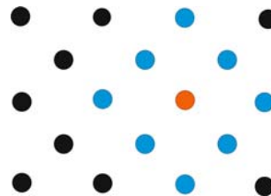
Fig. 2. Points with equal Manhattan distance
