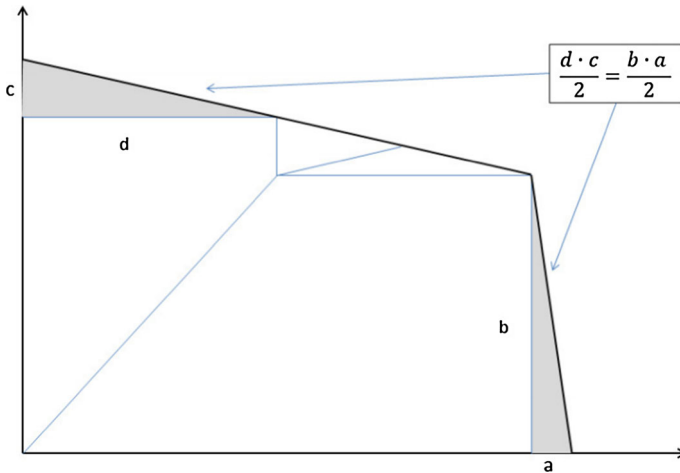
Fig. 3 A two dimensional example of A(t, s)
