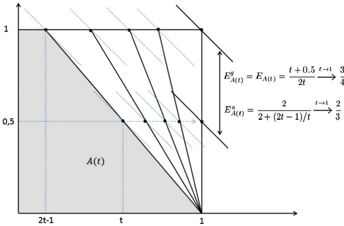
Fig. 2 Two dimensional examples to show the tightness
