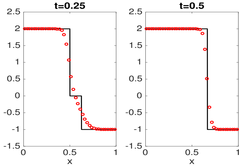
FIGURE 5. Example (6.6). Jin-Xin method without defect measure corrections. Solid line : exact solution; circles : numerical solution.
