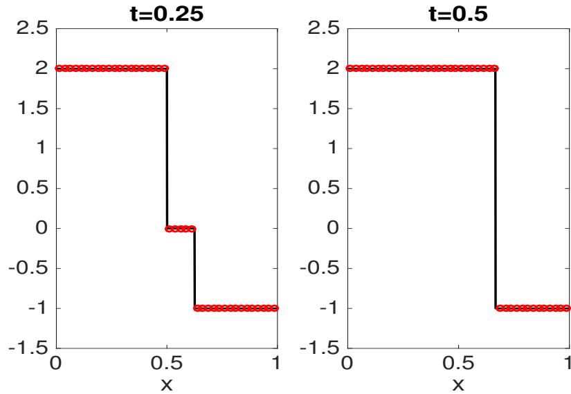
FIGURE 7. Example (6.6). Algorithm 4.2: Jin-Xin method with defect measure corrections based on the anti-diffusive law (3.62) for a general non-linear flux. Solid line : exact solution; circles : numerical solution.
