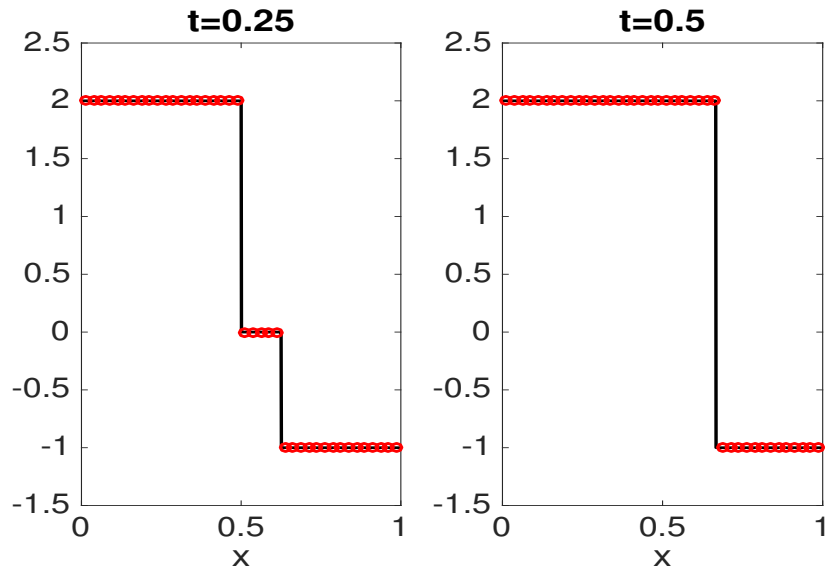
FIGURE 6. Example (6.6). Algorithm 4.1: Jin-Xin method with defect measure corrections based on the anti-diffusive law (3.62) for a general non-linear flux. Solid line : exact solution; circles : numerical solution.
