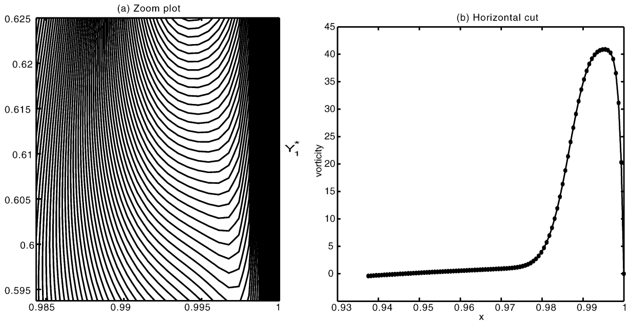
Fig. 8. Vorticity plot at the first critical time t = T_1^* . (a) Zoom plot in the region [63/64, 1] \times [19/32, 5/8] ; same convention as in Fig. 5(a). (b) Vorticity profile along the horizontal cut y = Y_1^* = 0.6107 near the first bifurcation point.
