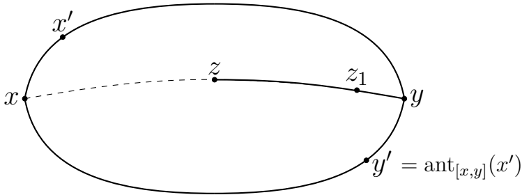
Fig. 3. The interval [x, y] and z \in [x, y] with d(z, y) = j \geq 2 and z_1 \in [z, y] \cup S_1(y) .
