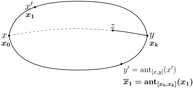
Fig. 2. The interval [x, y] with the re-labelled vertices in bold, and z \in [x_0, x_k] \cap B_1(x_k) .
