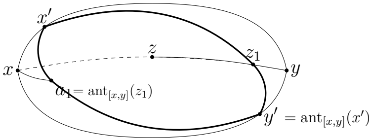
Fig. 4. Picture for Case z_1 \sim y' . The bold cycle represents the fact that a_1 and z_1 are antipoles w.r.t. not only [x, y] but also [x', y'] .
