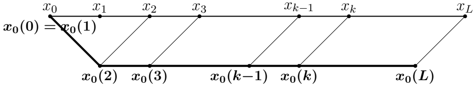
Fig. 1. Transport geodesic g_{x_0} (along g ) shown in bold.
