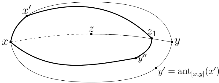
Fig. 5. Picture for Case d(z_1, y') = 2 . The bold cycle represents y'' = \text{ant}_{[x, z_1]}(x') .
