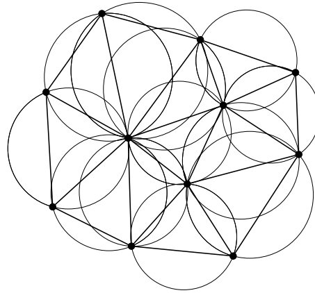
Figure 1. A Delaunay triangulation.
