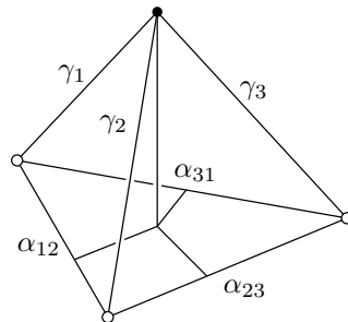
Figure 14. Tetrahedron with one ideal and three hyperideal vertices, partitioned into four special pyramids
