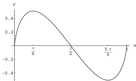
Figure 5. Milnor’s Lobachevsky function, y = \mathbb{J}(x) .
