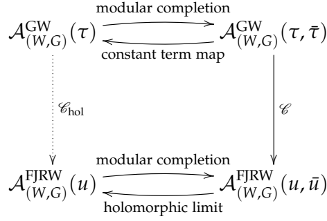
Figure 3: LG/CY correspondence
