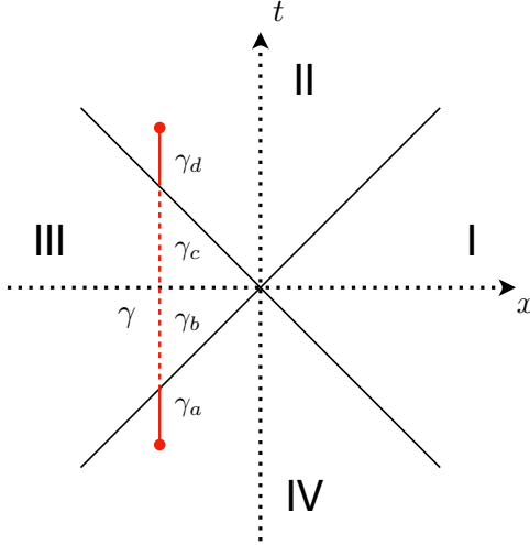
Figure 4: Four regions of a two-dimensional slice of Minkowski space. The Bondi coordinates with r > 0 cover only region II and part of region III. When r \in (-\infty, \infty) , the Bondi coordinates cover regions II, III, and IV. We also show the image of the bench under the map (D.4). For small J , the bench \gamma = \gamma_a \cup \gamma_b \cup \gamma_c \cup \gamma_d ends in Region II and IV. The segment in the middle is dashed as it corresponds to analytically continued complex coordinates (u, r, \phi) .
