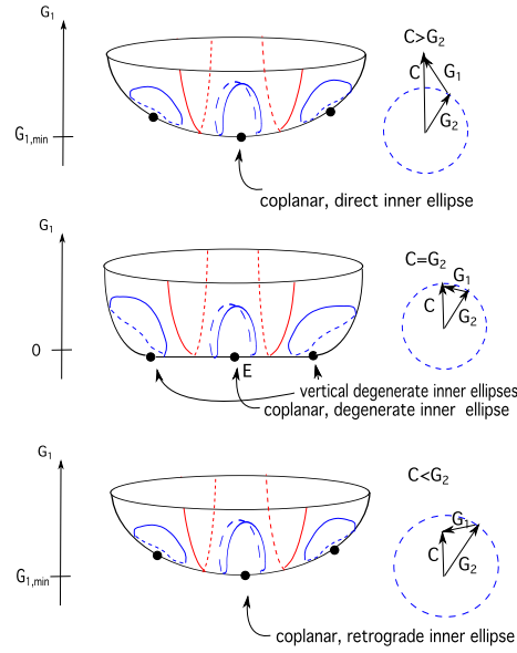
FIGURE 5.1. The reduced quadrupolar flow near the “bottom” \{G_1 = G_{1,\min}\} . We are interested only in the regions near the depicted coplanar equilibria inside the separatrices.
