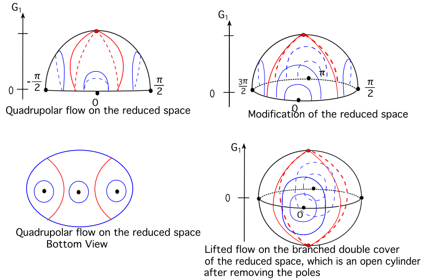
FIGURE 7.1. The flow foliation on the reduced space with C = G_2 and its branched double cover.
