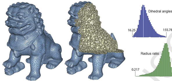
Figure 1: An example of our tetrahedral meshing result on the Lion model (input 100K triangles). Left and middle are the meshing result (55K vertices and 300K cells) and a cutaway view, respectively. Right are the dihedral angle and radius ratio distributions.
