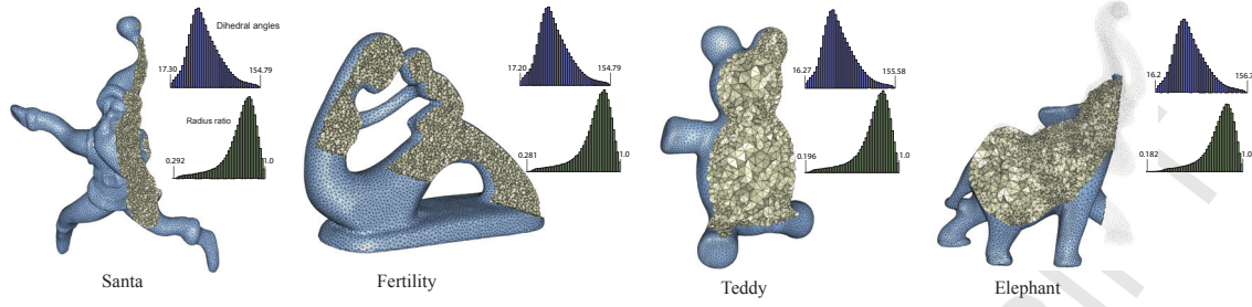
Figure 6: Tetrahedral meshing results of our algorithm. The two images of the left (Santa and Fertility) are uniform meshes, and the two images of the right (Teddy and Elephant) are graded meshes.
