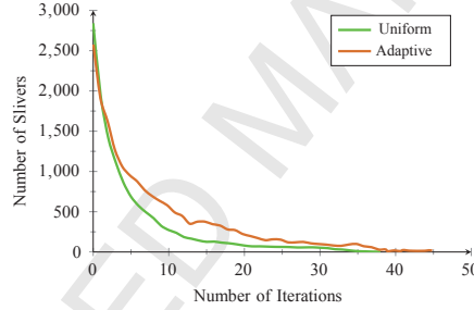
Figure 8: Number of slivers in relation to the number of iterations. The statistics are obtained on the Santa (uniform with 136K tetrahedra) and Elephant (adaptive with 133K tetrahedra) models.
