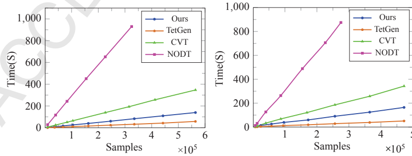
Figure 9: Performance comparison of our method with tetGen, CVT and NODT. Left: uniform tetrahedral mesh; right: graded tetrahedral mesh. The running time of our algorithm also contains building the uniform grid.
