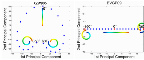
Figure 4: Visualization of blended cylinder from -360^\circ to 360^\circ using dimensionality reduction to 2D. Left: result of deformation gradient [XZWB06], right: result of [BVG09].
