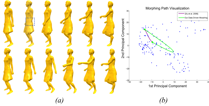
Figure 9: Comparison of dancer morphing results using the dataset from [VBMP08]. (a) the result of [XZWB06] (top) and our method (bottom), (b) visualization of morphing using feature coordinates and dimensionality reduction to 2D. Purple: [XZWB06]; Green: our data-driven morphing.
