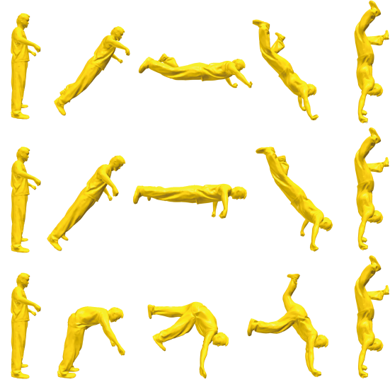
Figure 10: Morphing results using the handstand dataset from [VBMP08]. First row: [HAWG08], second row: existing data-driven morphing [GLHH13], third row: our data-driven morphing.
