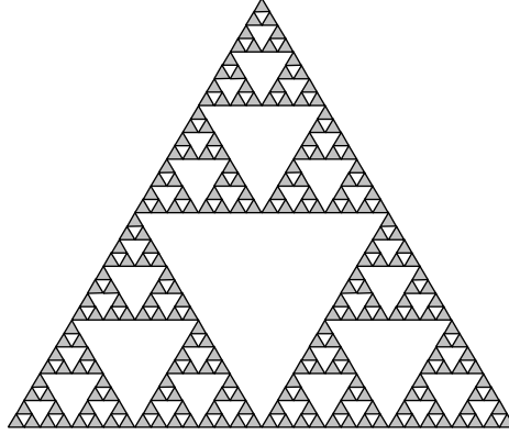
FIGURE 4. Construction of the Sierpinski gasket: after 5 steps.
