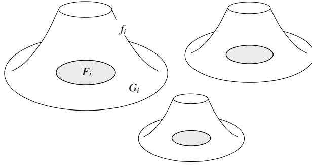
FIGURE 10. Capacitors (F_i, G_i) and their test functions.
