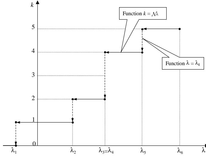
FIGURE 3. Sample graphs of functions \lambda \mapsto \mathcal{N}_\lambda (horizontal) and k \mapsto \lambda_k (vertical)
