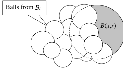
FIGURE 6. Choosing ball B(x, r) : the measure of the shaded region is larger than \alpha .
