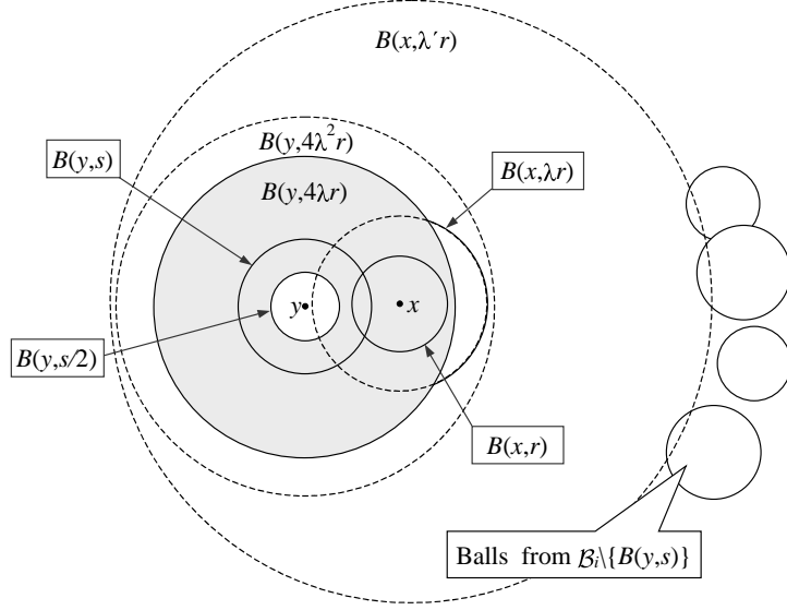
FIGURE 9. The annulus \tilde{a} = A(y, \frac{1}{2}s, 4\lambda r) is shaded.
