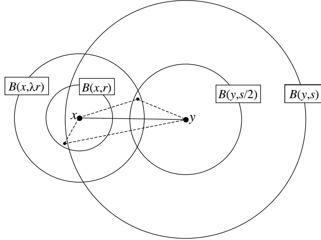
FIGURE 5. Illustration to Lemma 3.8
