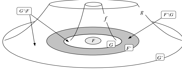
FIGURE 1. Capacitor (F' \setminus G, G' \setminus F)
