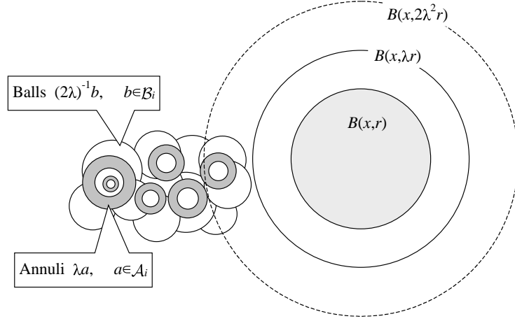
FIGURE 7. Ball B(x, \lambda r) does not intersect \frac{1}{2\lambda}b , whereas the union of all \lambda a is covered by the union of all \frac{1}{2\lambda}b .
