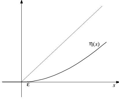
FIGURE 13. A function \eta(s)
