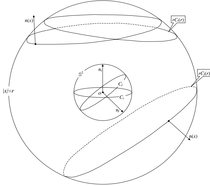
FIGURE 11. Circle C_i with multiplicity 2 and circle C_j with multiplicity 1.
