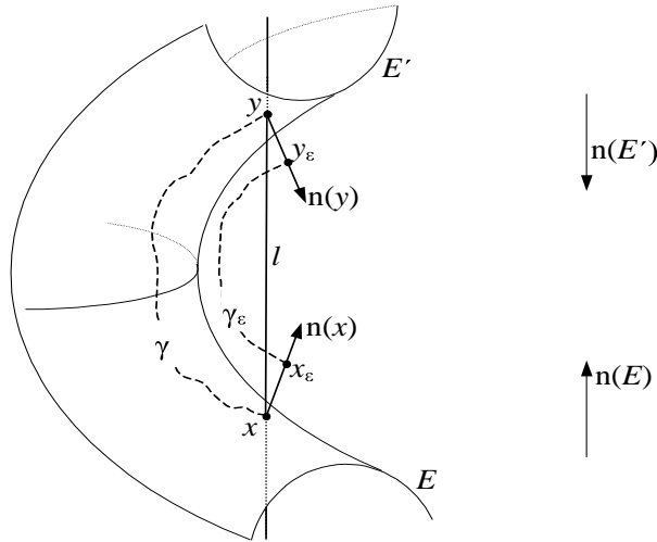
FIGURE 16. Paths \gamma and \gamma_\varepsilon .
