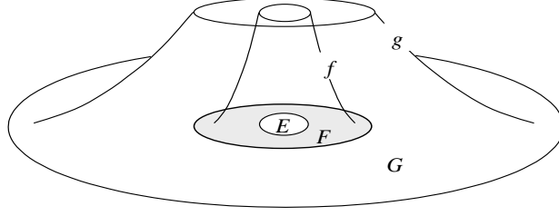
FIGURE 2. Capacitors (E, F) and (F, G)
