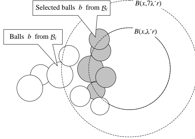
FIGURE 8. The selected balls (shaded) are inside B(x, 7\lambda'r) .
