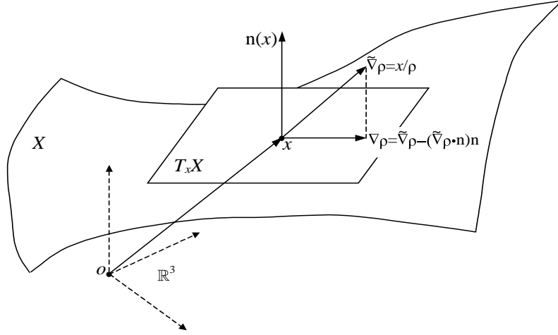
FIGURE 12. Gradients \nabla\rho and \tilde{\nabla}\rho
