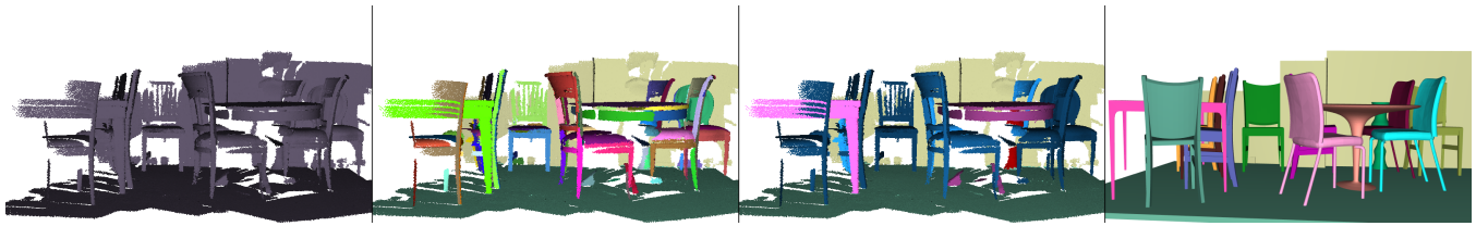
Figure 2: A zoom into the cluttered region of Figure 1 (left), reveal that accurate segmentation and classification are challenging, even for human perception. We initially over segment the scene (mid-left) and search-classify meaningful objects in the scene (mid-right), that are reconstructed by templates (right) overcoming the high clutter.
