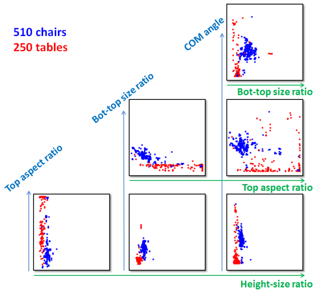
Figure 6: Visualization of joint distribution of several feature pairs using our RDF classifier, showing clear separation between chairs (blue) and tables (red).
