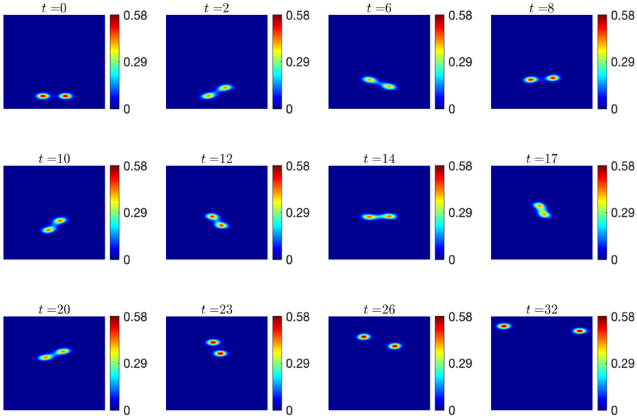
Fig. 10. (Color online) Plots of |u^\epsilon(x, y, t)|^2 at different times for Case (iii) in region [-9, 9] \times [-5, 32] .
