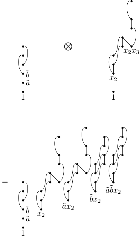
FIG. 10. The \mathcal{A}_2(1) -module structure of H^*(\mathbb{B}\mathbb{Z}_8, \mathbb{Z}_2) \otimes H^*(\mathbb{B}^2\mathbb{Z}_2, \mathbb{Z}_2) . The dashed lines indicate an (2, 8) -Bockstein. Each dot indicates a \mathbb{Z}_2 , the short straight line indicates a \text{Sq}^1 , the curved line indicates a \text{Sq}^2 .
