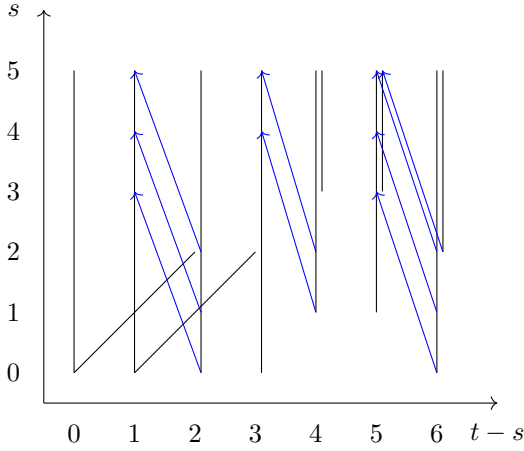
FIG. 11. \Omega_*^{\text{Spin}}(\mathbb{B}\mathbb{Z}_8) . The arrows indicate differentials. Note that there is a nontrivial extension at t - s = 5 , the result is \Omega_5^{\text{Spin}}(\mathbb{B}\mathbb{Z}_8) = \mathbb{Z}_8 \times \mathbb{Z}_2 , which has already been calculated in [42] and [43].
