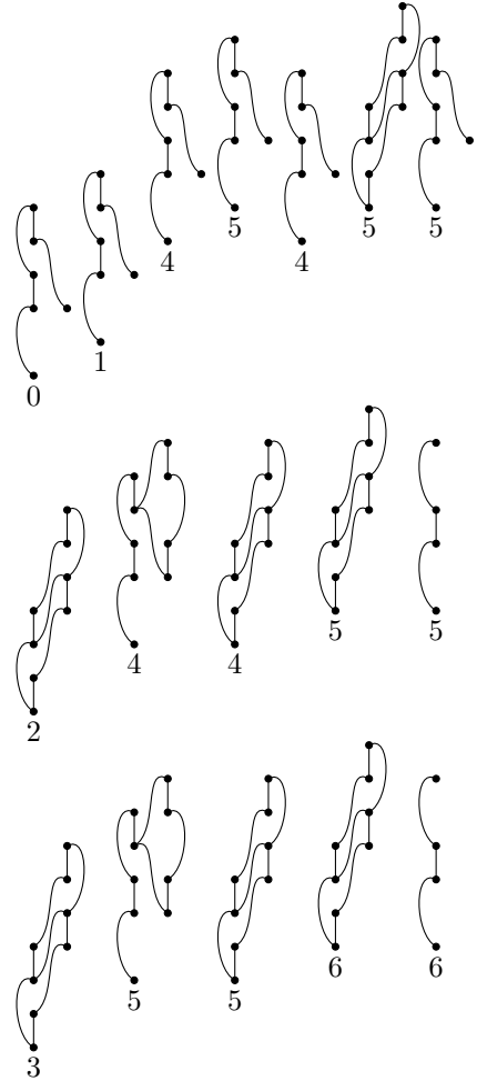
FIG. 7. The \mathcal{A}_2(1) -module structure of H^{*+3}(MSO(3), \mathbb{Z}_2) \otimes H^{*+2}(MZ_4, \mathbb{Z}_2) \otimes H^*(B^2\mathbb{Z}_2, \mathbb{Z}_2) . Each dot indicates a \mathbb{Z}_2 , the short straight line indicates a Sq^1 , the curved line indicates a Sq^2 . Each label indicates its degree.
