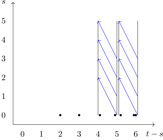
FIG. 9. (\Omega_*^{\text{Spin} \times_{\mathbb{Z}_2} (\text{SU}(2) \times_{\mathbb{Z}_2} \mathbb{Z}_8)}(\mathbb{B}^2 \mathbb{Z}_2)) / (\Omega_*^{\text{Spin} \times_{\mathbb{Z}_2} (\text{SU}(2) \times_{\mathbb{Z}_2} \mathbb{Z}_8)}) . The arrows indicate differentials.
