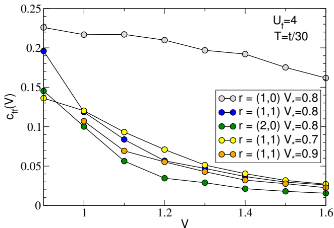
FIG. 10. (Color online) Spin correlations between local electrons, c_{\text{ff}}(r) , for near neighbors (1,0), (1,1) and (2,0). c_{\text{ff}}(r) grows as V approaches the AF-singlet crossover. The temperature T = t/30 . The f -orbital on-site repulsion U_f = 4 .
