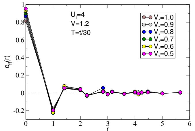
FIG. 9. (Color online) f - f electron spin correlation function c_{ff}(r) for bulk hybridization V = 1.2 and different impurity hybridizations V_* . As V_* decreases the short-range AF order with near neighbor (1,0) becomes deeper. The temperature T = t/30 . The f -orbital on-site repulsion U_f = 4 .
